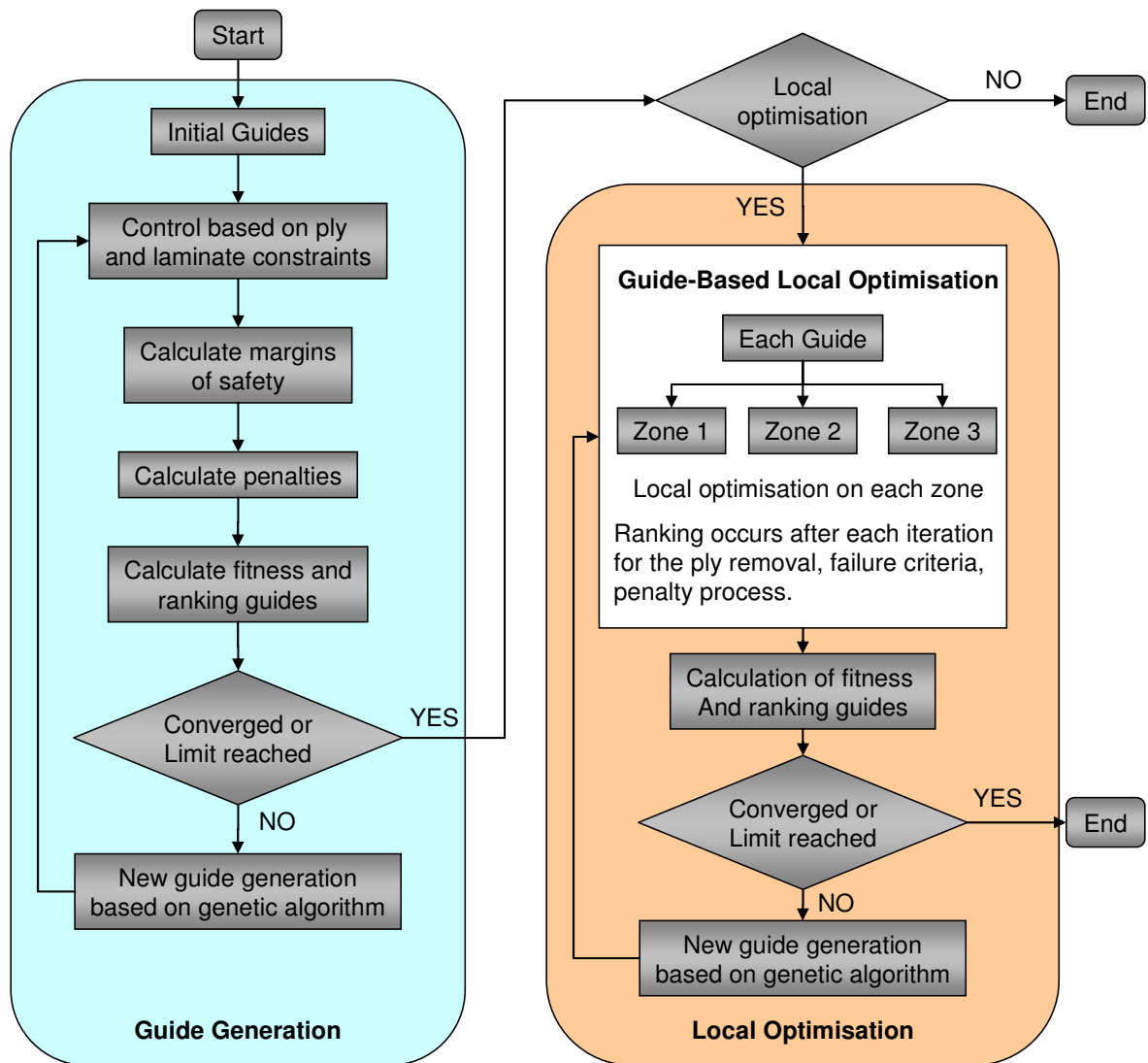
Figure 1. Process Flow
